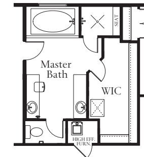
Partial second floor level with opt. master bath
